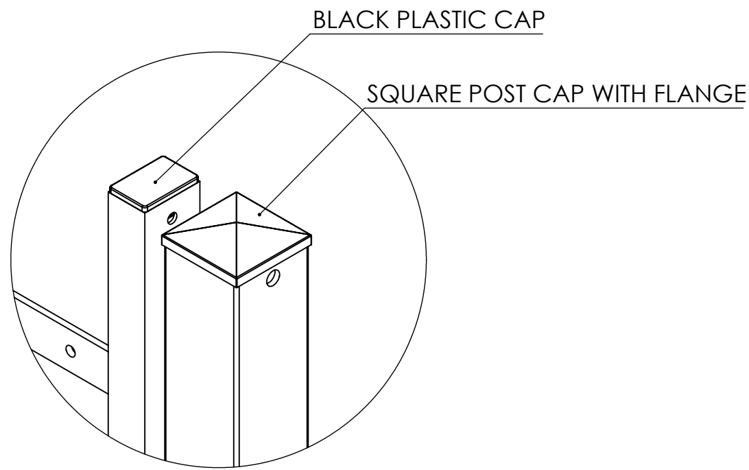
Gate & Post Attachment Example
