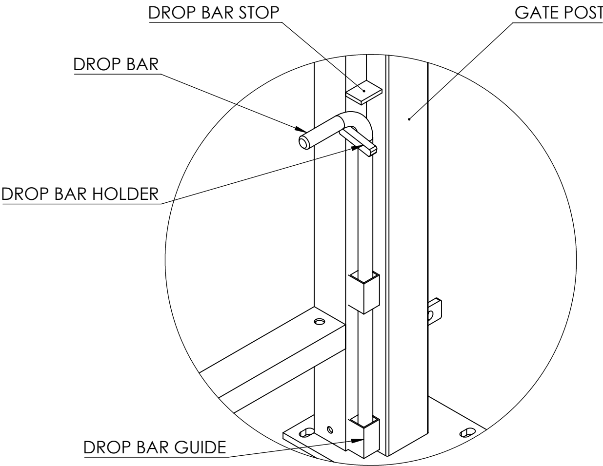
Back View of Drop Bar & Guides
