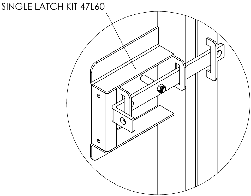
Slide Latch With Padlock Holes & Reversible Handle As Standard. (Padlock Not Included)
